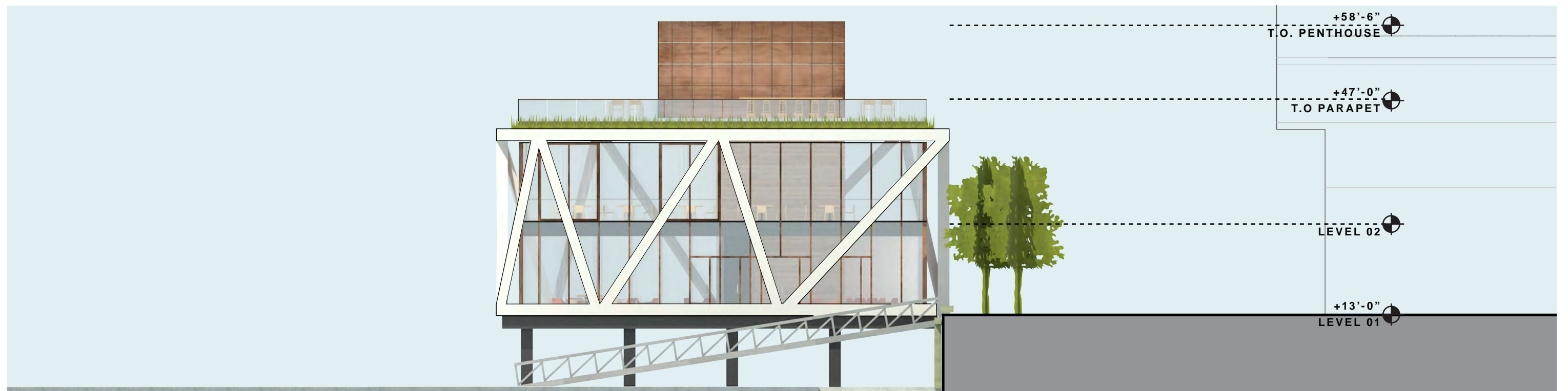
WATER BUILDING 1: EAST ELEVATION
